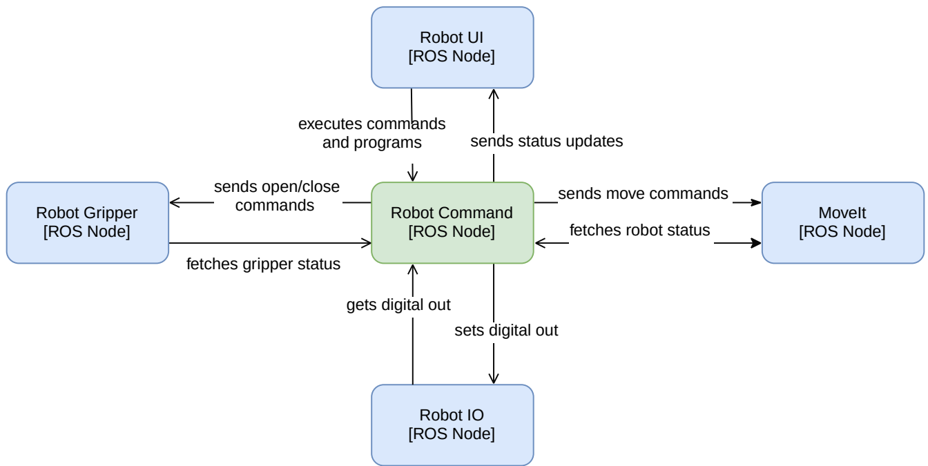
Figure 1. TMC Script - Container Diagram
