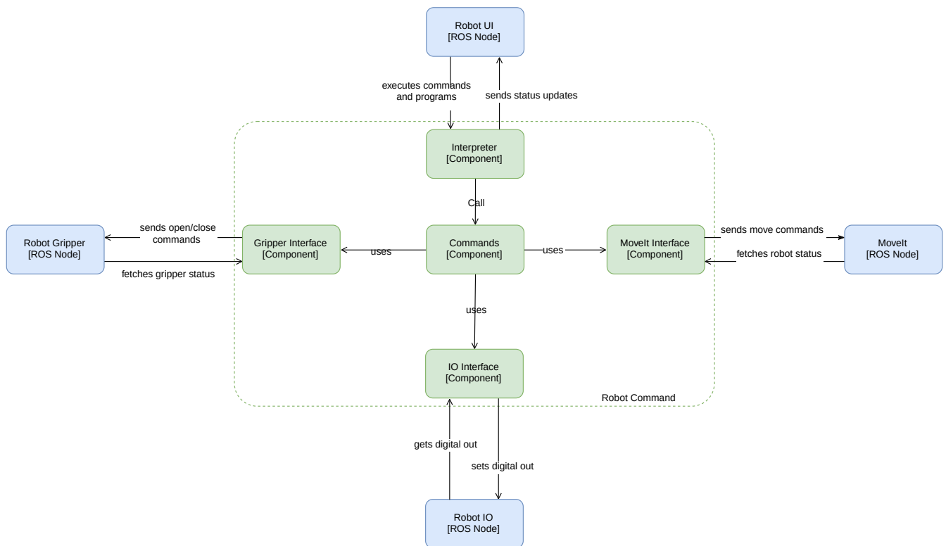
Figure 2. TMC Script - Component Diagram
